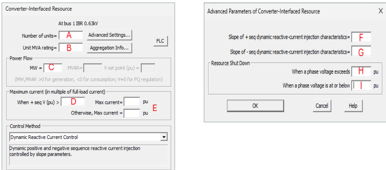
Figure 15 Converter-Interfaced Resources
